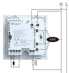
Connection 4: 2-pipe ON/OFF +Tio2/ESP
