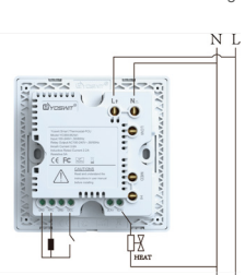
Connection 6: Underfloor heating
