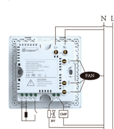
Connection 7: Water source heat pump
