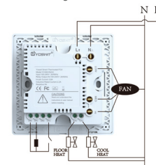
Connection 3: 2-pipe ON/OFF +floor heating
